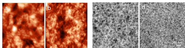
Figure 2. Morphology of PTNT:PC 71 BM blends. AFM height images (left) and TEM bright-field micrographs (right) of the active layer in photovoltaic devices of (a,c) 2:3 PTNT:PC 71 BM and (b,d) 2:3 PTNT:PC 71 BM processed with 3% DIO. Root-mean-square values of 1.6 \pm 0.2 \text{ nm} . The scale bar is representative for all images.
